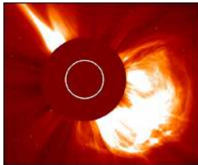
Solar flares of 4 th November 2003 (NASA)
