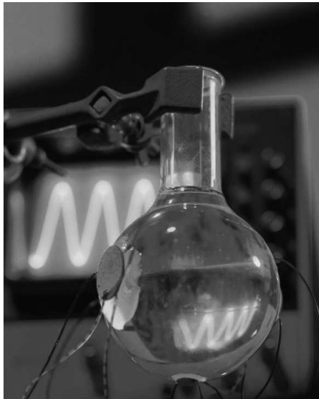
sonoluminescentie experiment
